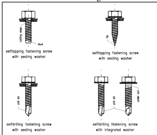
Figure 1: Fastening screws for metal members and sheeting
